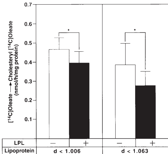
Fig. 6. Cholesteryl ester formation stimulated by either VLDL or d < 1.063 g/ml lipoproteins. Plasma was obtained from either APOEKO (open bar) or LPL/APOE KO (closed bar) mice (n = 5) which had been fed an atherogenic diet for 8 weeks. VLDL or d < 1.063 g/ml lipoproteins were isolated from pooled plasma by ultracentrifugation. Thioglycollate-elicited peritoneal macrophages were prepared from wild-type C57BL/6 mice. After treatment with LPDS for 24 h, the cells were incubated with 12.5 mg/ml of the indicated lipoproteins for 24 h, and cholesteryl ester formation was determined as described in Experimental Procedures. Errors bars denote SD; * P < 0.05 (n = 3).
